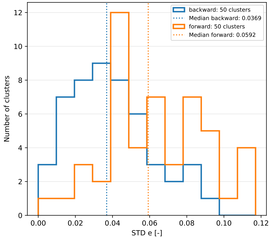
K=50 | Within-cluster STD distributions | Each cluster counts once
